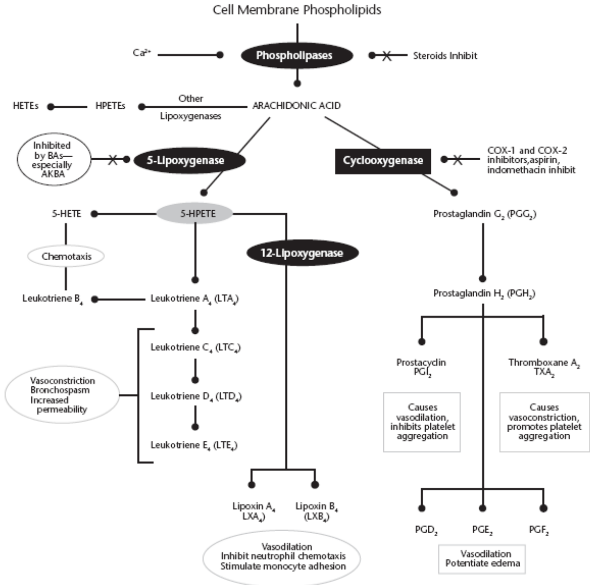
Generation of arachidonic acid metabolites and their roles in inflammation.
